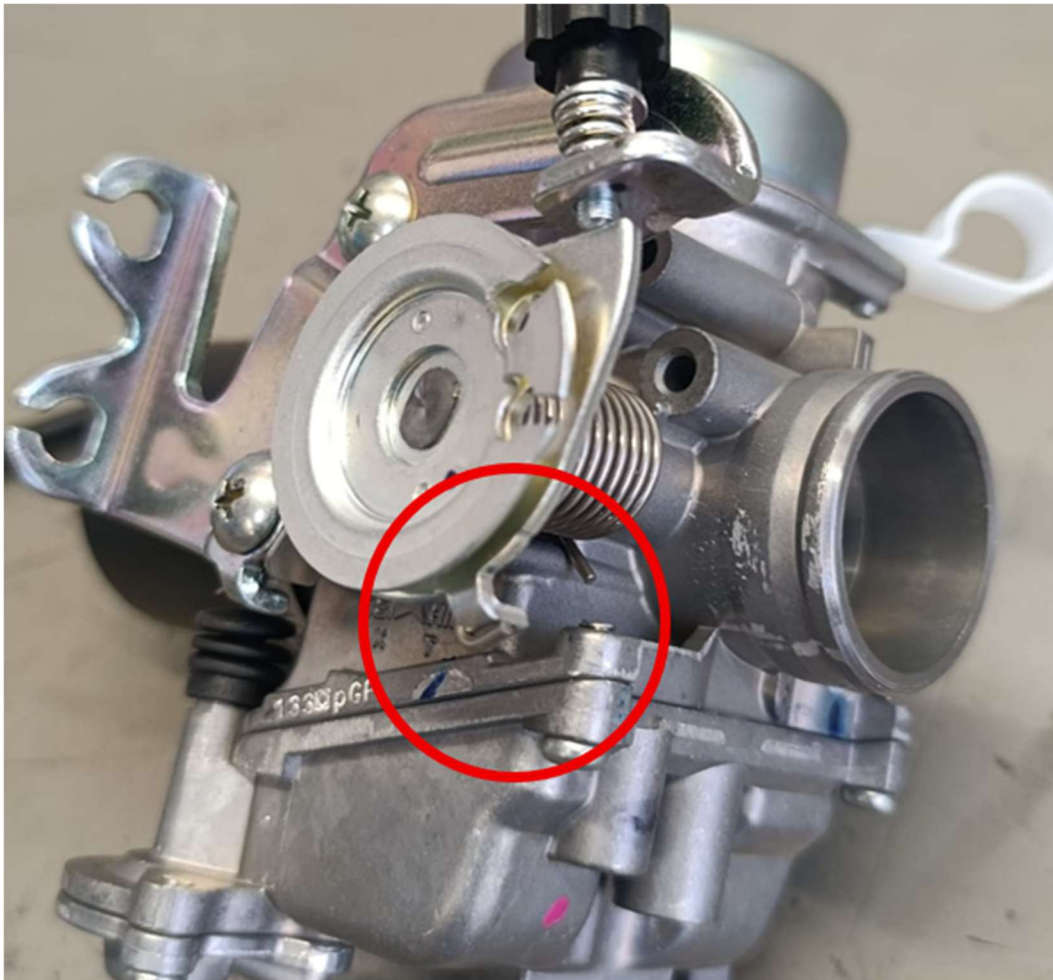
Original mounting point of the throttle body return spring
